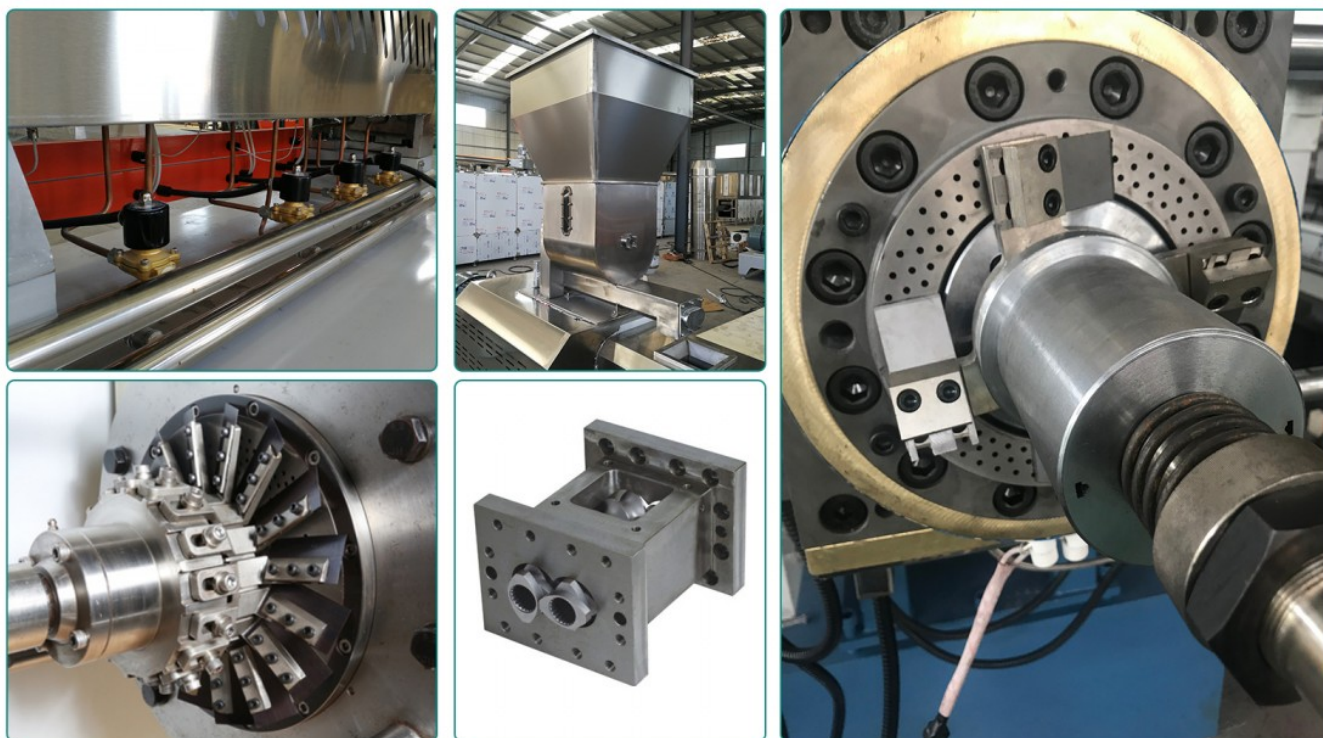
(Soya Nuggets Machine Detailed Pictures)
